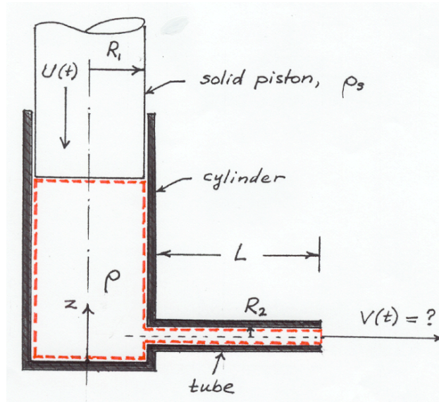
Fig. 1: The system and the control volume (broken red line) for Methods 1 and 2. This control volume is fixed in the inertial reference frame of the cylinder.
